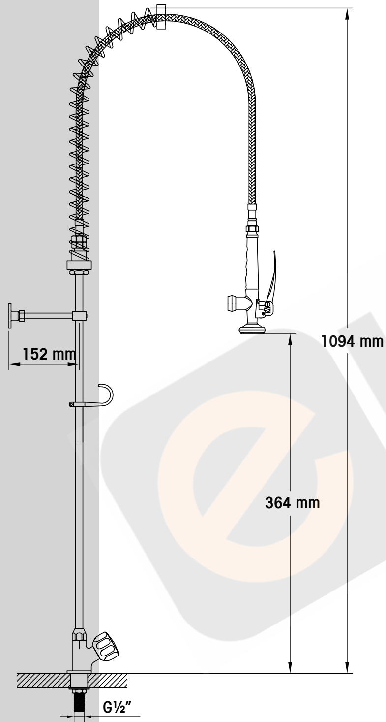
SOPORTE PARED DUCHA Ref. 15505
