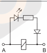
C: Variantes 3, 5, 54 LED (AC)
