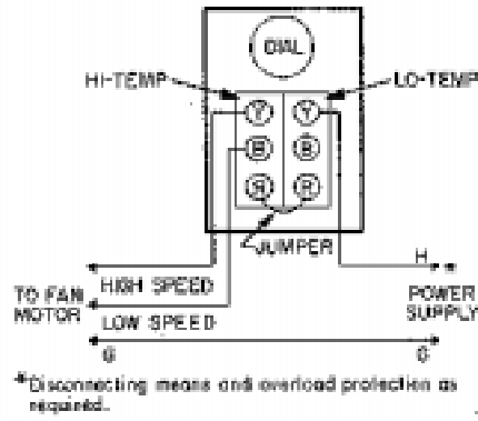
Fig. 8: An A28AA shows typical wiring for the control of a two speed ventilating fan. When control temperature reaches the dial setting, the low temperature switch starts the fan on low speed. If the space temperature continues to rise, the high temperature switch supplies power to the high speed motor winding while disconnecting to the low speed winding.
