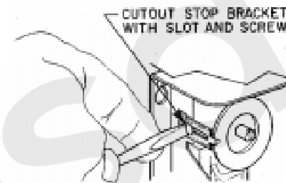
Fig. 4: The thermostats have a screw type cutout stop. The stop screw must be loosened and moved to the stop setting desired. Tighten screw after setting is made.
